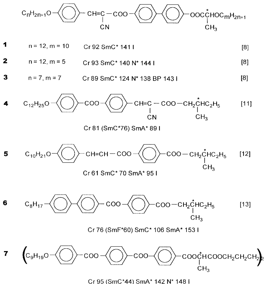
Scheme. Chemical structures and phase transitions of the liquid crystal materials used in the mixtures.
